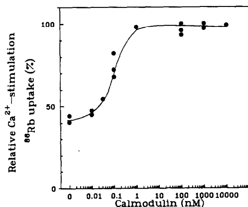
Fig.1. Effect of direct calmodulin addition on the \text{Ca}^{2+} -activated \text{K}^+ channel. Protein from luminal plasma membrane vesicles was solubilized and reconstituted into phospholipid vesicles as described in section 2. ^{86}\text{Rb}^+ uptake into the vesicles was measured in the presence and absence of 1\text{ }\mu\text{M} free \text{Ca}^{2+} at increasing concentrations of calmodulin. The \text{Ca}^{2+} -dependent ^{86}\text{Rb}^+ uptake was calculated for each concentration of calmodulin in % maximum ^{86}\text{Rb}^+ uptake.
