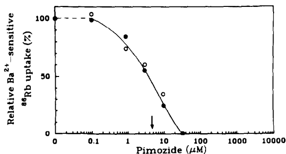
Fig.2. Effect of pimozide on the \text{K}^+ channel activity in plasma membrane vesicles ( \circ ) and reconstituted vesicles ( \bullet ). The \text{Ba}^{2+} -sensitive ^{86}\text{Rb}^+ uptake into the vesicles was measured after 10 min as before [7] with increasing concentrations of pimozide. The K_{0.5} for the inhibition is indicated by an arrow. Pimozide was added from a stock solution in DMSO. The final concentration of DMSO was 2% and did not affect the ^{86}\text{Rb}^+ uptake. 100% activity corresponds to 110\text{ pmol } ^{86}\text{Rb}/\text{mg protein per min} .
